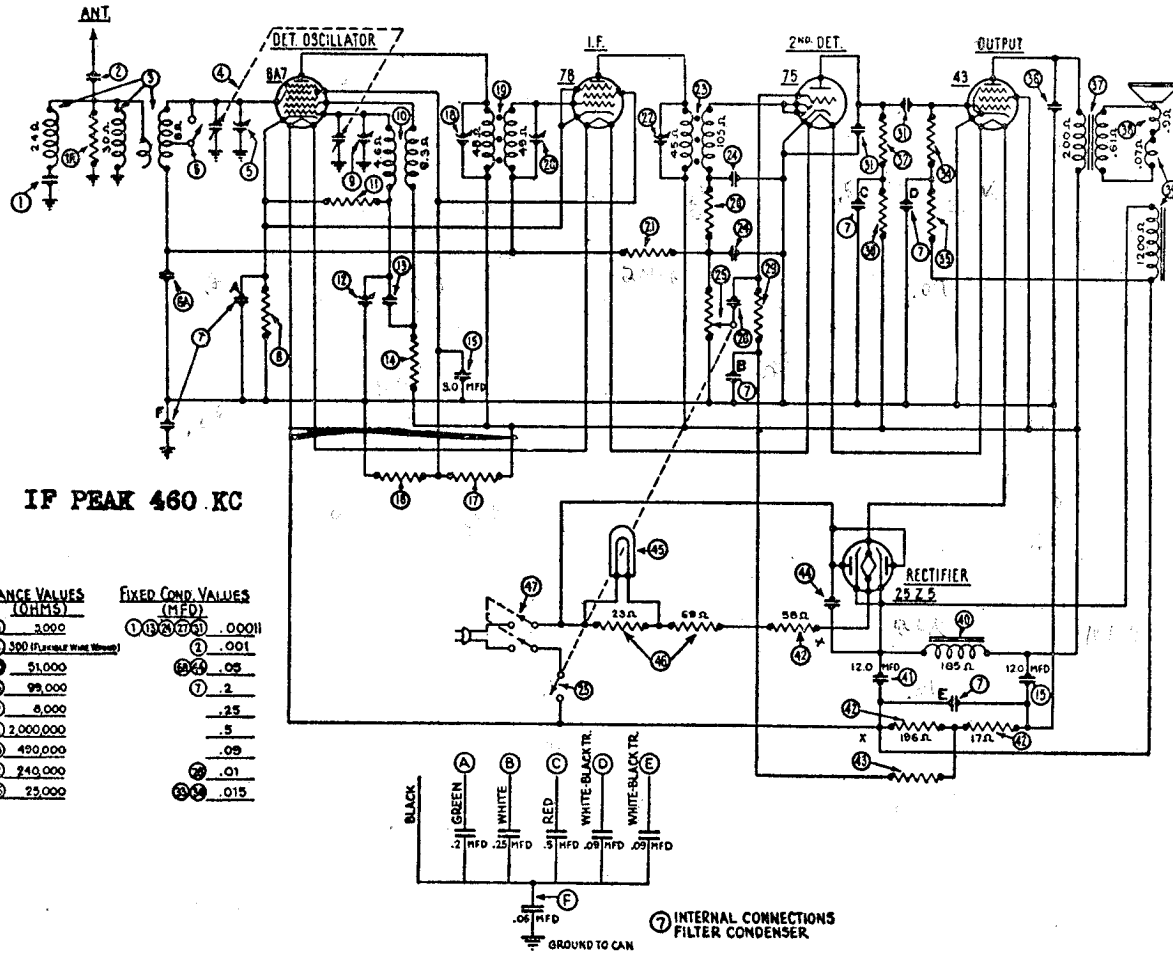
Fig. 3—Schematic Wiring Diagram
